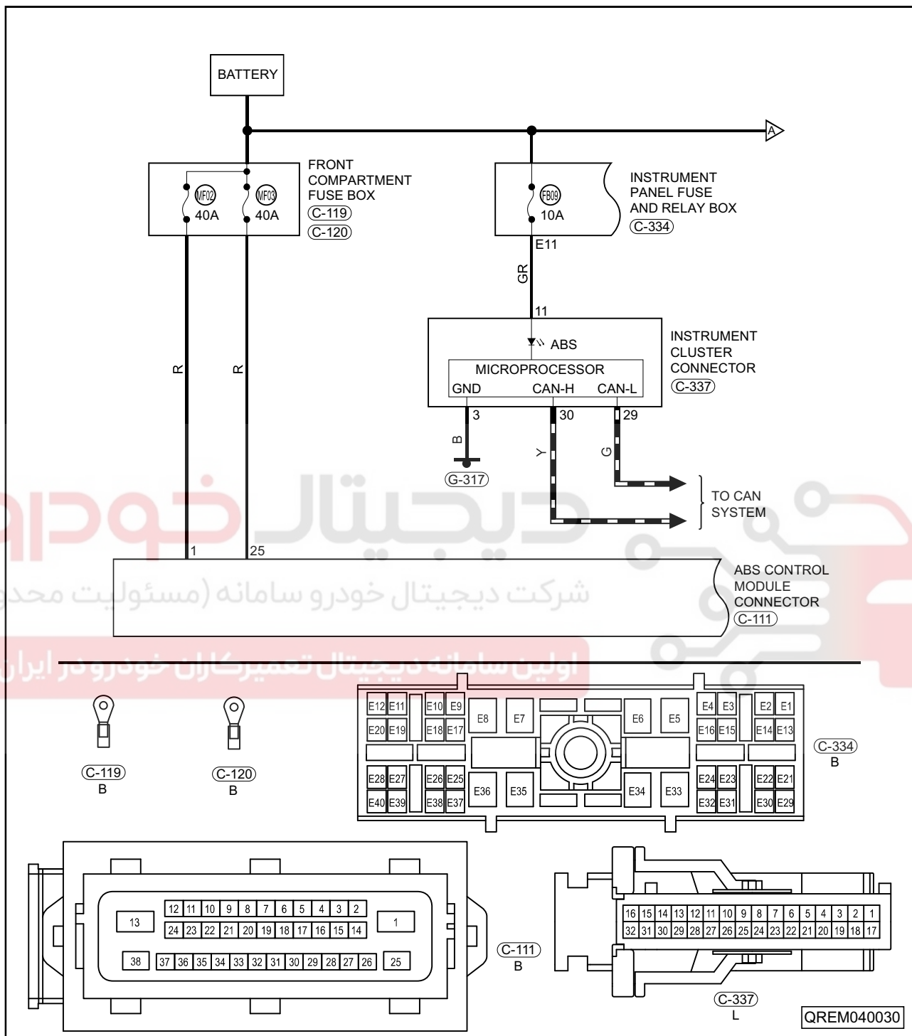
ABS circuit diagram (page 1)
