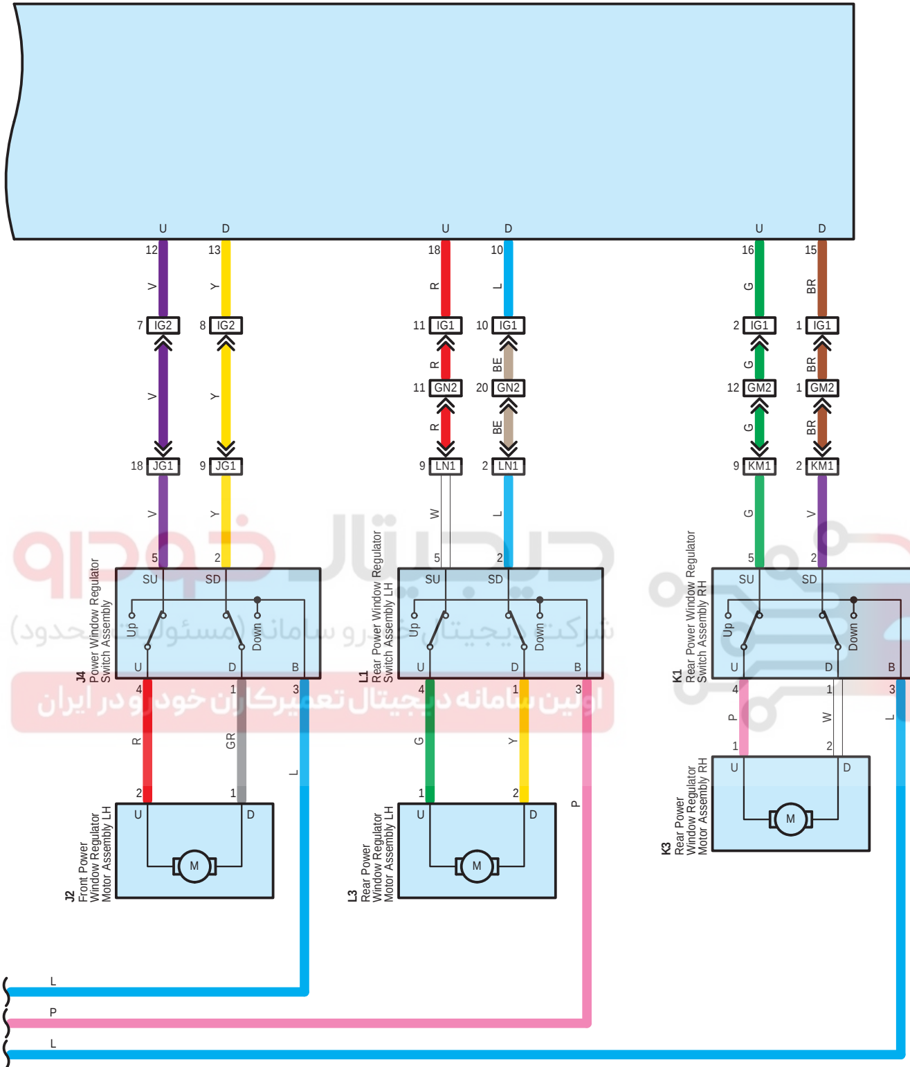
15 Power Window Regulator Master Switch Assembly
