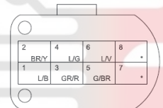
AT transmission fluid temperature sensor & speed sensor
