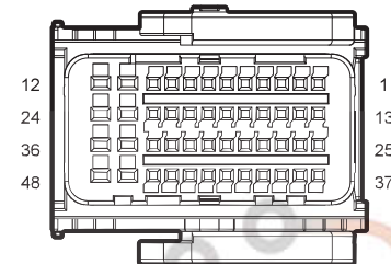
F01 BCM C2
