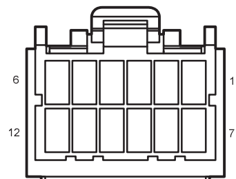
M23 Gear Shifting(CVT) Harness Connector
