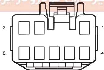
D33 Right Front Door Switch (Low Spec)
