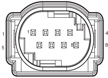
W04 Tailgate Close Switch
