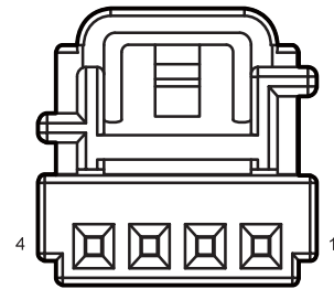
D19 Left Rear Door Switch (High Spec)
