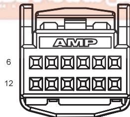
M07 Clock Spring -Horn
