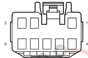
D31 Left Rear Door Switch (Low Spec)
