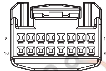
M04 Central Switch
