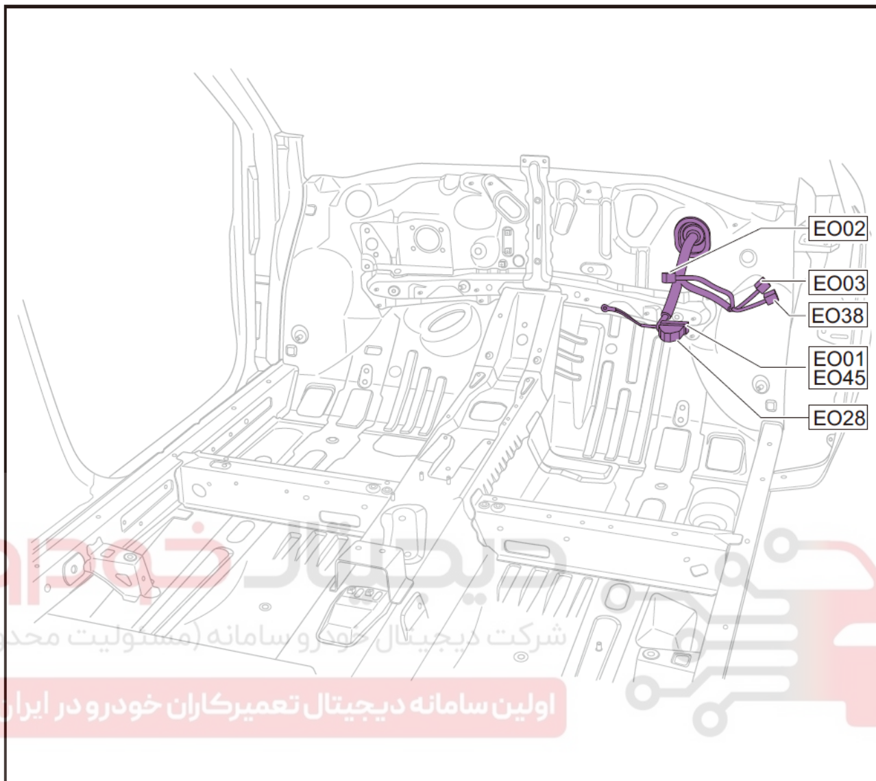
Engine Harness Layout Drawing (Continued) (JED-4013)
