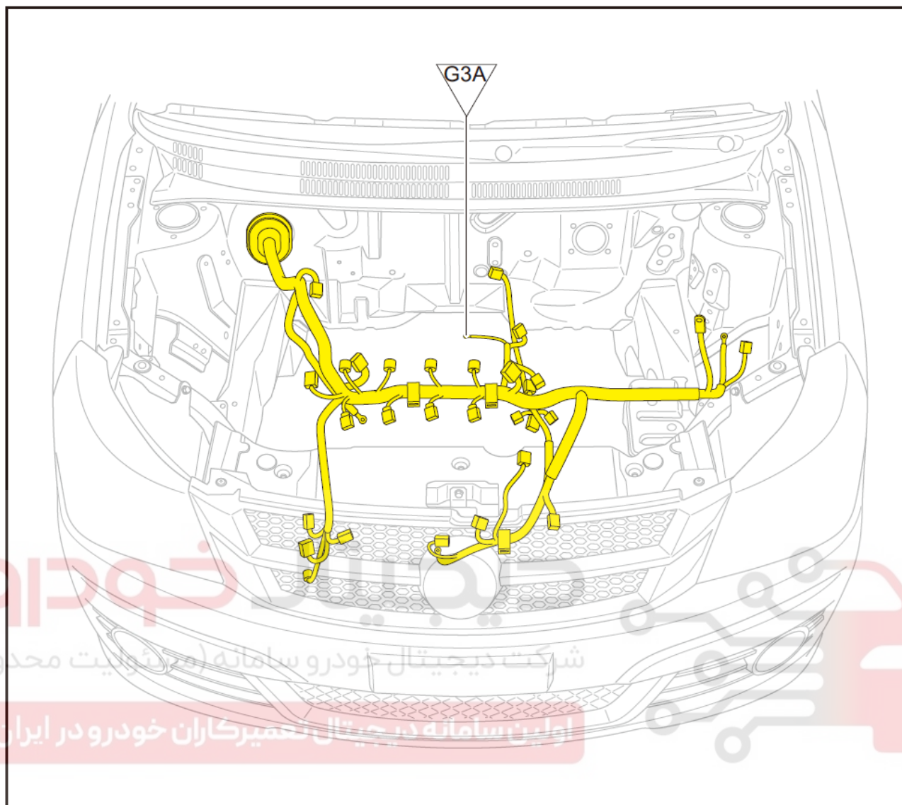
Engine Grounding Point Layout Drawing (Continued) (JED-4013)
