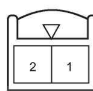
Harness connector of fuel injection nozzle 3 EO21
