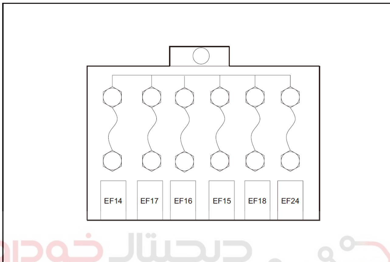
Frontal view of Engine Compartment Fuse (JED-4G13, 14K4/5QA)
