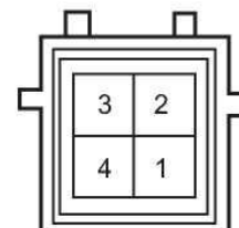
Engine oil pressure switch harness connector EO30
