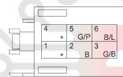
Hazard warning lamp switch
