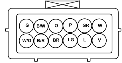
B2-03 Gearshift plug (I)
