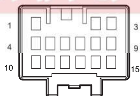
I_BRRD Body W.H. Connector Connecting RR Door W.H.
