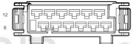
F04 Glass Regulating Controller 2
